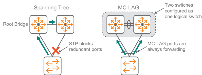
Figure 16 Traditional spanning tree vs MC-LAG
