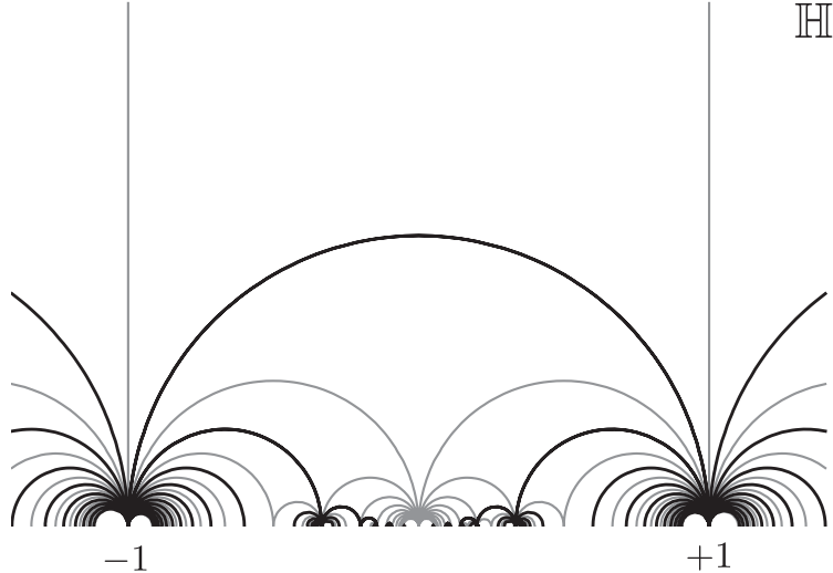
FIG. 1. The tessellation by \Gamma_\theta and its sub-tessellation by \Gamma_\infty \setminus \Gamma_\theta . The thick lines are where phase transitions in supergravity can occur.
