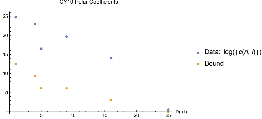
FIG. 4. Here, we plot the polar coefficients of Z_{RR}^{d=10} .
