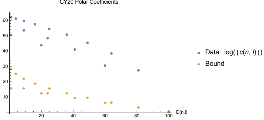
FIG. 5. Here, we plot the polar coefficients of Z_{RR}^{d=20} .
