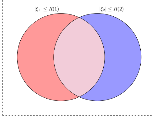
FIG. 9. Here, we show an image from Dr. John Venn [42]. The LHS of (B.7) for N = 2 is represented by the white, blue, and red parts. The RHS is the sum of two terms: blue and white, and red and white. Thus, the sum is greater than the LHS.
