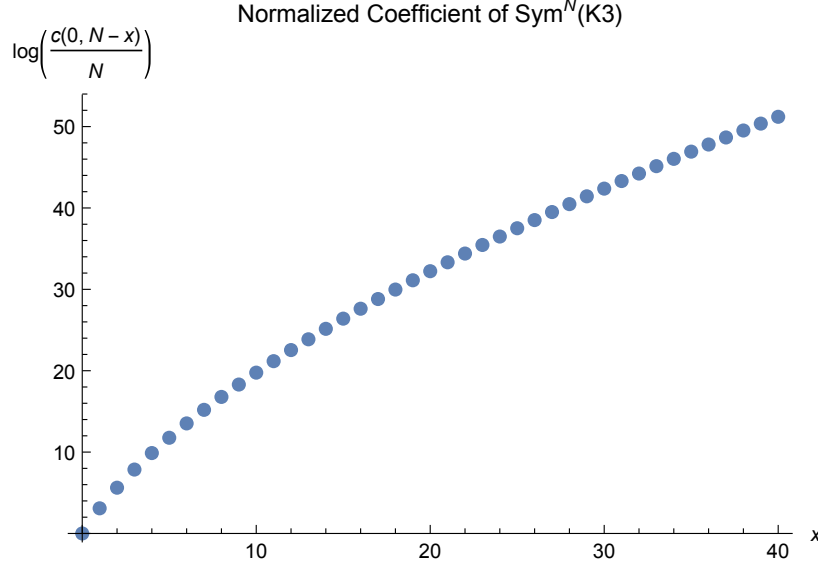
FIG. 8. Here, we plot the normalized coefficients of y^{N-x} terms in elliptic genus of \text{Sym}^N(K3) for x = 1, \dots, 40 in the large N limit. Note the subexponential growth in the plot. Numerical values for the first twenty terms are given in Table I.
