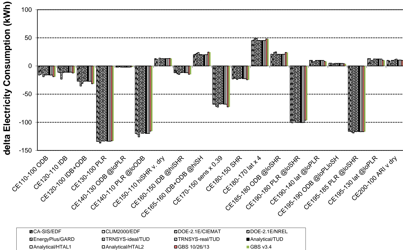
Figure B16.5.1-9. HVAC BESTEST: Indoor (Supply) Fan Electricity Sensitivities
