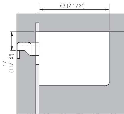
Fixture for cabinet
