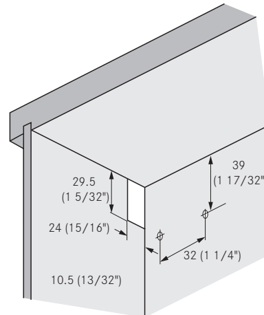
Fixture for cabinet
