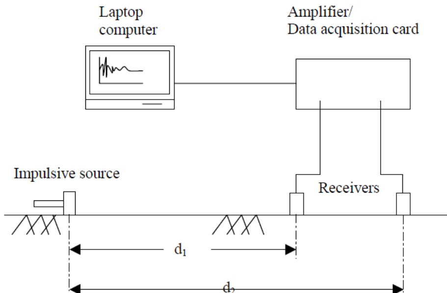
Fig. 0-9 Surface Wave analysis system, after [Hildebrand, 2002]
