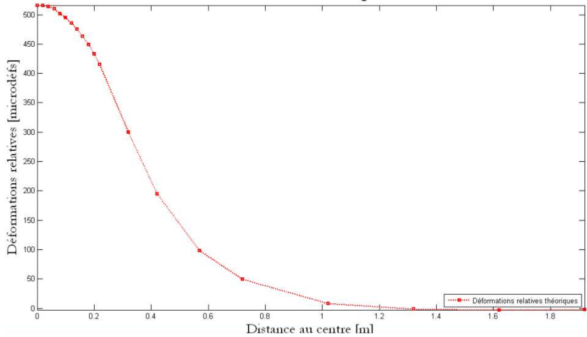
Figure 6 Direct calculation; numerical vertical strain (top of UGA) basins; S_2 structure; pseudo-static method
