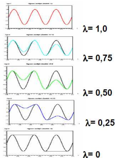
Fig. 0-33 Complex deformations signals applied to the sample; multi-peak experiment, after [Merbouh 2007]
