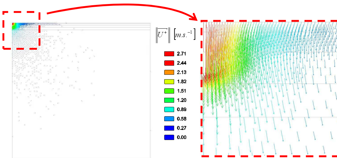
Fig. 3-24 Velocity field \vec{U}^+ obtained after the shock
