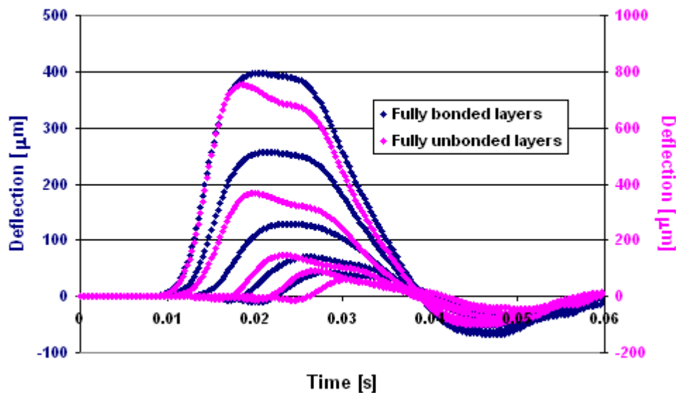
Fig. 3-46 Comparison between bonded and unbonded configurations, dynamic method
