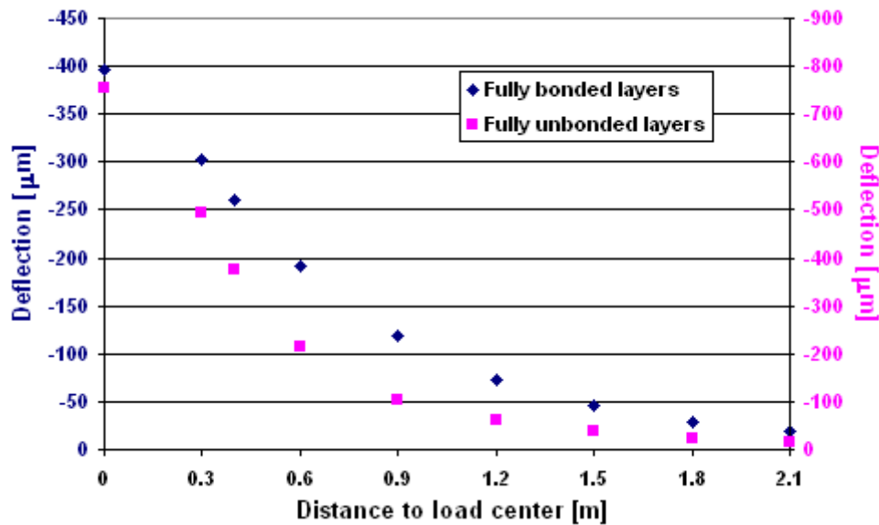
Fig. 3-45 Comparison between bonded and unbonded configurations, pseudo-static method
