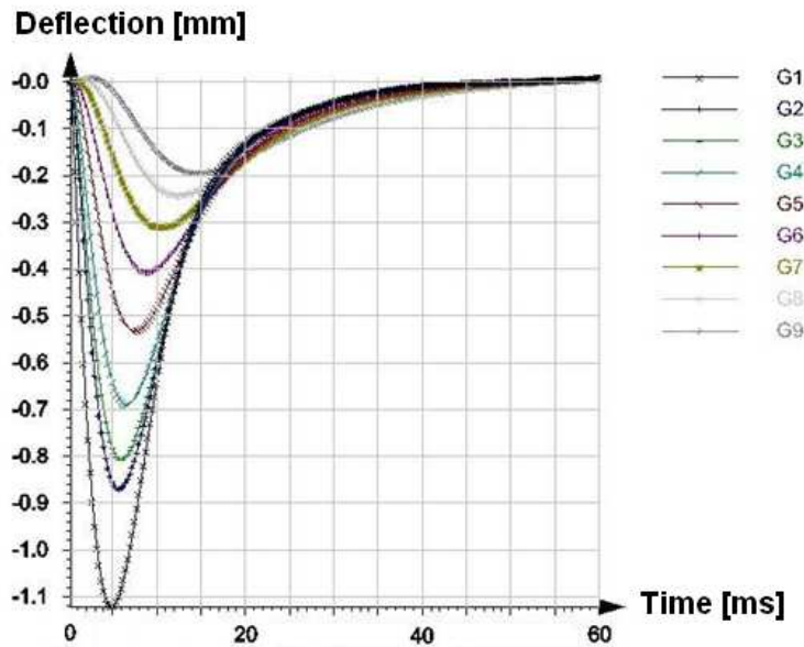
Fig. 3-25 Time-related deflections from M_1 modelling
