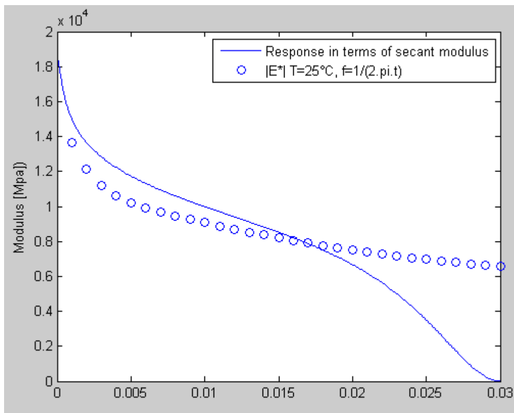
Fig. 3-44 Secant modulus of S_2 AC 2 material under sinusoidal load; after Viscoanalyse
