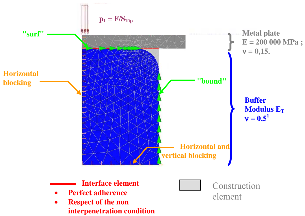
Fig. 1-10 Finite Elements modelling of the buffer behaviour under axial loading
