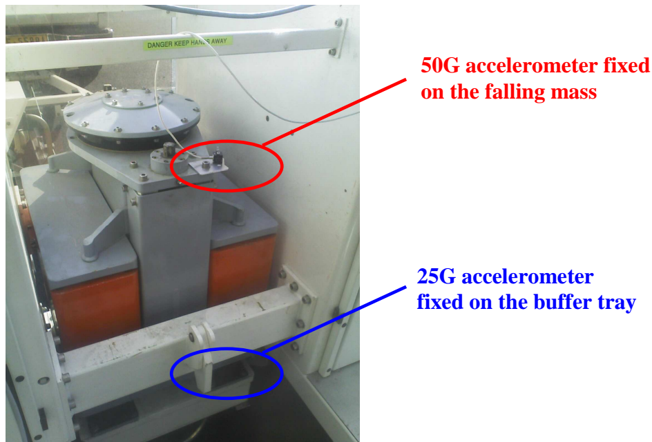
Fig. 1-12 Test setup related to the accelerometer-based mass motion study
