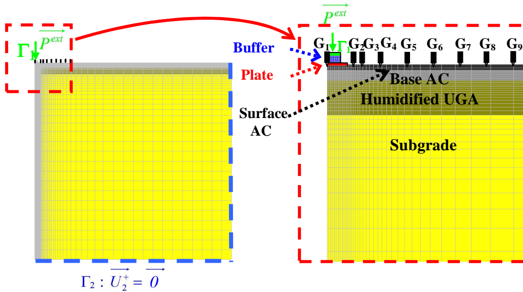
Fig. 2-2 Mesh discretization; shock model
