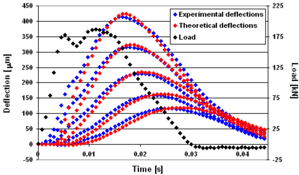
Fig. 3-38 Dynamic fitting with damping, S 3 structure, PI 1 test point
