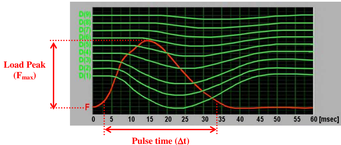
Figure 21 – Recording of the applied force and deflections
