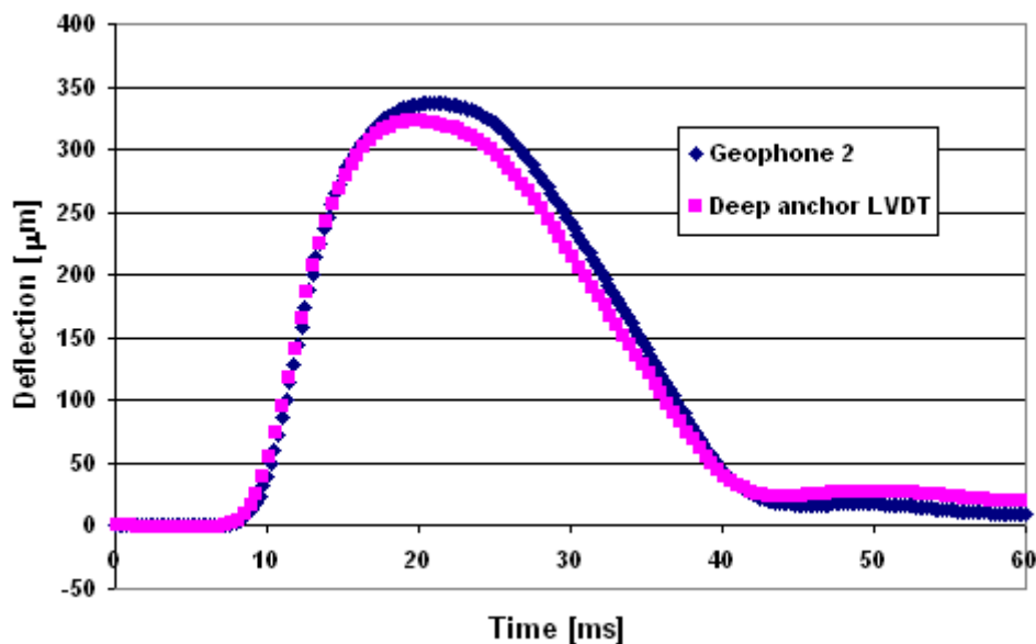
Fig. 1-33 Correlation between HWD and deep anchor surface deflection measurement; geophone 2
