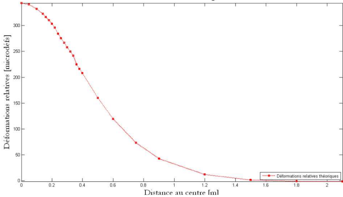
Figure 7 Direct calculation; numerical vertical strain (top of UGA) basins; S_2 structure; pseudo-static method
