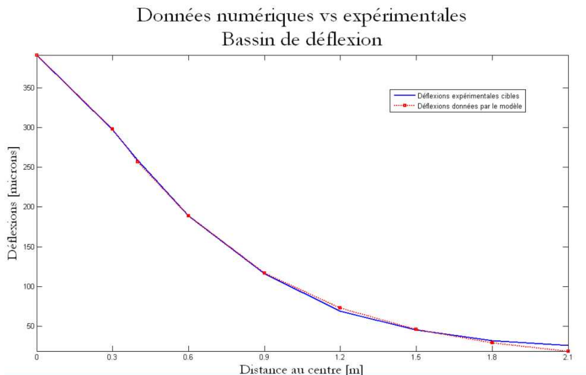
Figure 12 Backcalculation results; final fitting between numerical versus experimental deflection basins; S_2 structure; pseudo-static method
