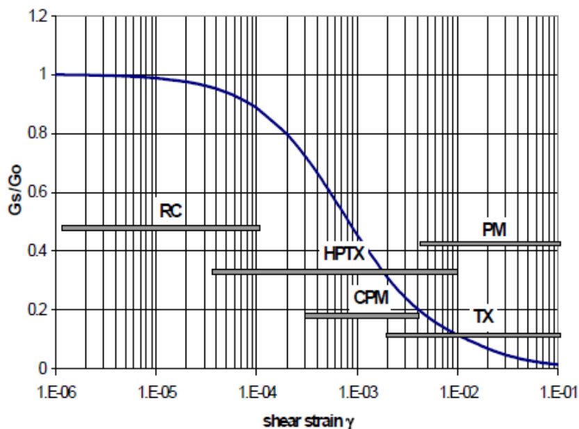
Fig. 0-11 Typical variation of normalized shear modulus as a function of shear strain (blue curve), after [Puech et al., 2004]
