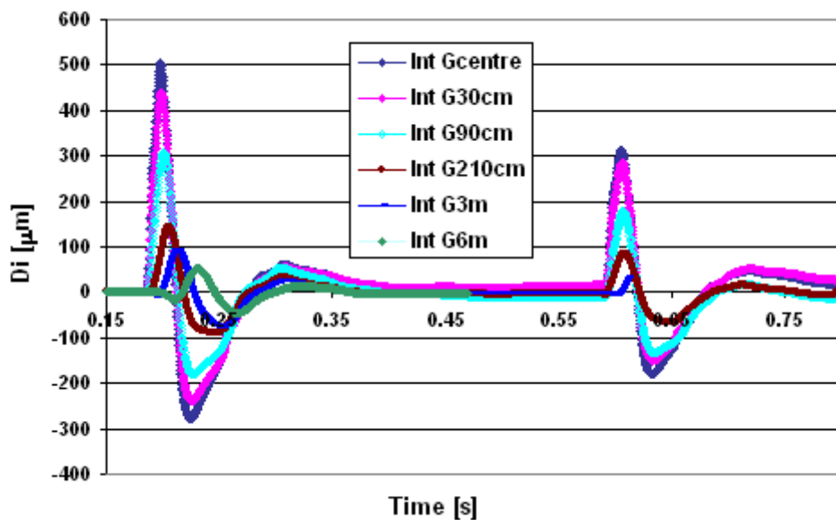
Fig. 1-45 Surface displacements at several distances from load centre; integration from geophone electrical signals (1/2)
