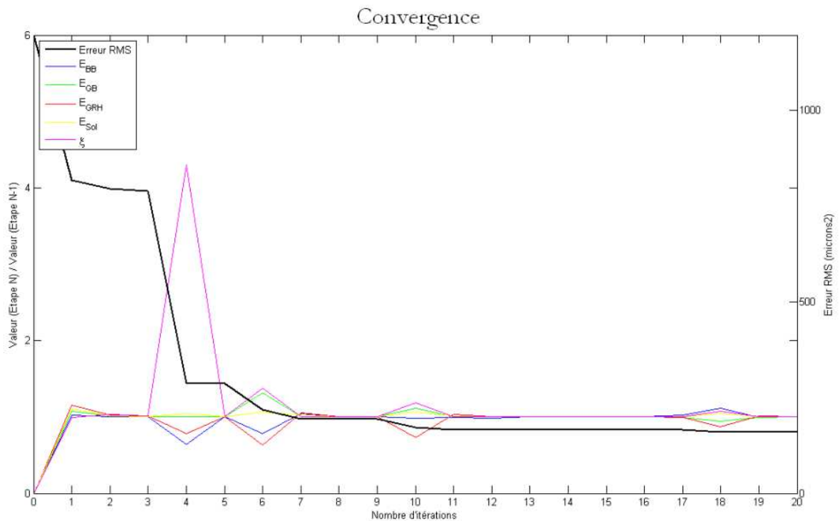
Figure 14 Backcalculation results; Stabilization of parameters and evolution of error with regard to iteration number; S_2 structure; dynamic method
