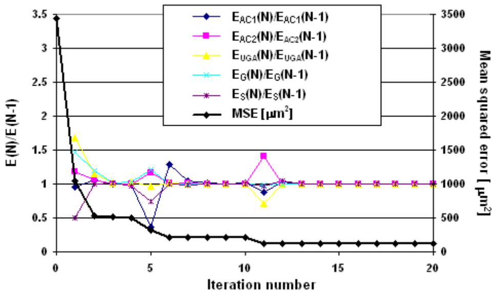
Fig. 3-39 Convergence in the dynamic case with damping, S 3 structure, PI 1 test point
