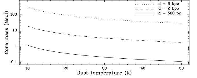
Fig. 11. Total gas plus dust masses in a core with 250 mJy integrated flux density at 870 \mu\text{m} ( 5\text{-}\sigma detection limit) as a function of dust temperature, for three typical distances: 500 pc (full line), 2 kpc (dashed line) and 8 kpc (dotted line).
