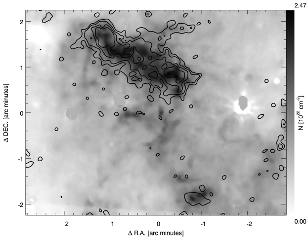
Fig. 13. Column density map of the IRDC G19.30+0.07, contained in the l = 19^\circ demonstration field. The map is derived from 8\ \mu\text{m} extinction values measured in the corresponding Spitzer/GLIMPSE map. The ATLASGAL emission at 870\ \mu\text{m} is overlaid in contours. The map center is at \alpha = 18^{\text{h}} 25^{\text{m}} 53.94^{\text{s}} , \delta = -12^\circ 05' 43.9'' (J2000), or l = 19.2771^\circ , b = +0.0703^\circ .
