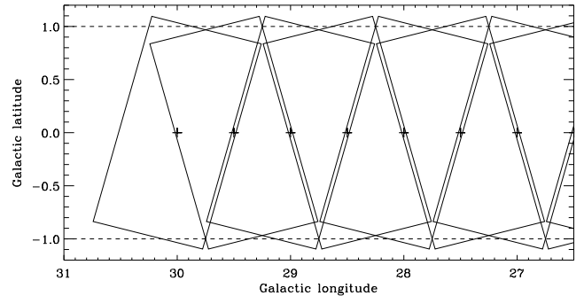
Fig. 2. Mapping strategy: each rectangular frame represents a single map. The plus symbols show the maps centers. A position angle of 15^\circ with respect to the galactic axis was chosen. Two neighboring maps are observed with position angles of +15^\circ and -15^\circ , respectively.
