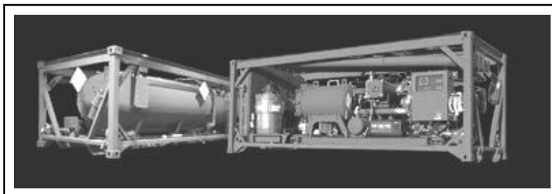
Figure 2-12. Modular fuel system
