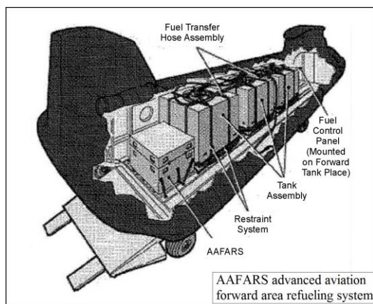
Figure 2-15. Extended range fuel system II functional components
