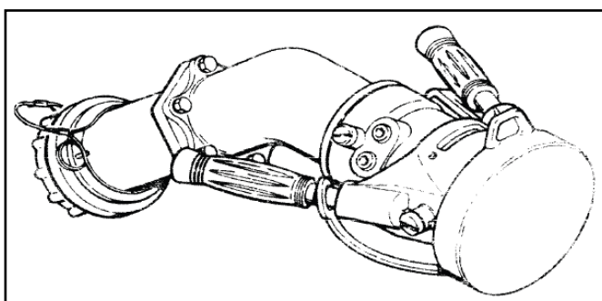
Figure 2-11. D-1 center point refueling nozzle
