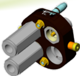
Multi connector Pressure-Return 65251
