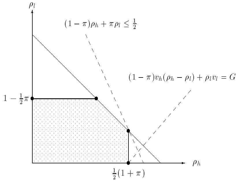
Figure 3: Optimal auction: optimal \rho 's
