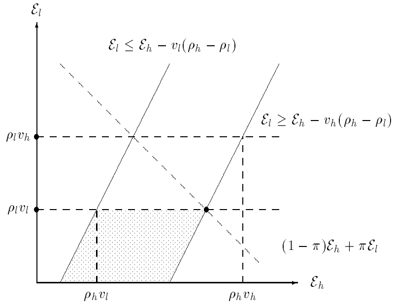
Figure 2: Optimal auction: optimal \mathcal{E} 's
