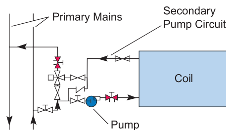
Primary-Secondary Connections
