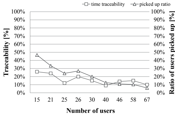
Figure 4. Traceability and picked-up ratio versus the number of users in large clusters.
