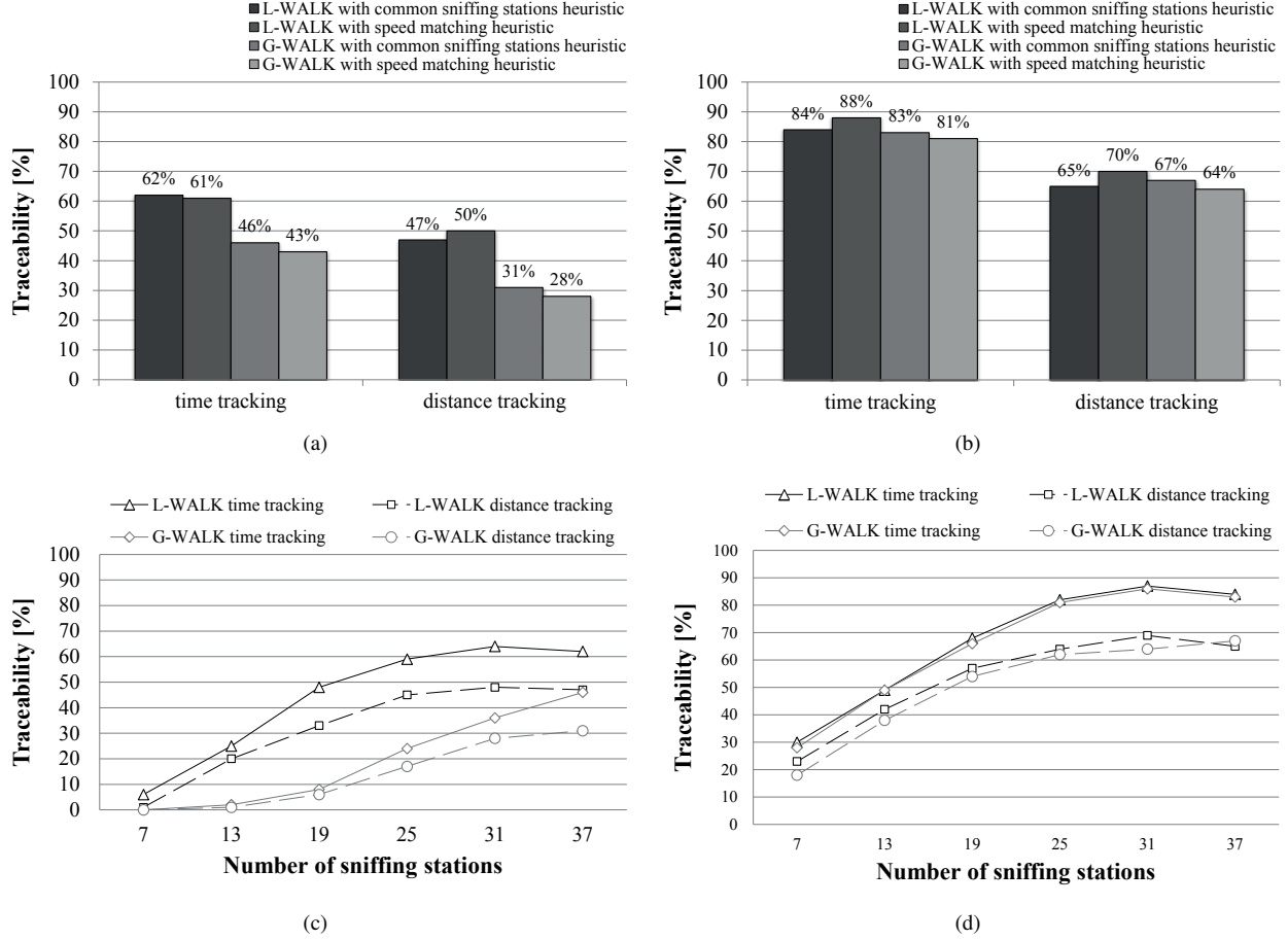
Figure 2. Traceability success: 2(a) single user tracking results; 2(b) multiple user tracking results. Adversary strengths using L-WALK and G-WALK: 2(c) single user; 2(d) multiple users.
