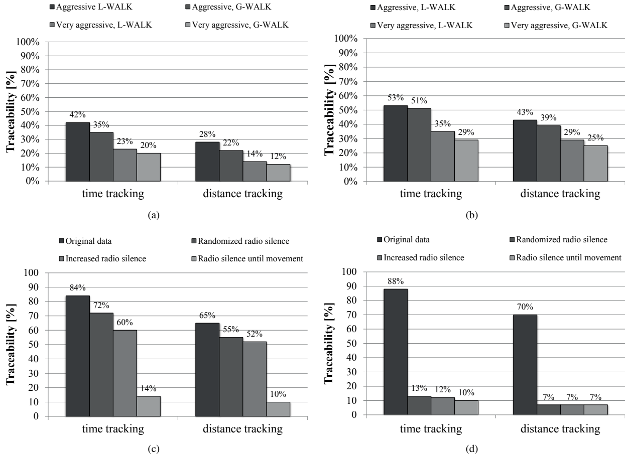
Figure 5. Results for aggressive parameters: 5(a) single user; 5(b) multiple users. Results with modified PCA in multiple user tracking: 5(c) common sniffing stations; 5(d) speed matching.
