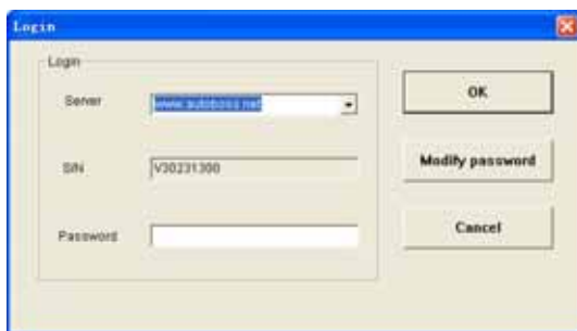
Fig 2-2 login interface
