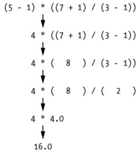
Figure 1-1. Evaluating an expression reduces it to a single value.
