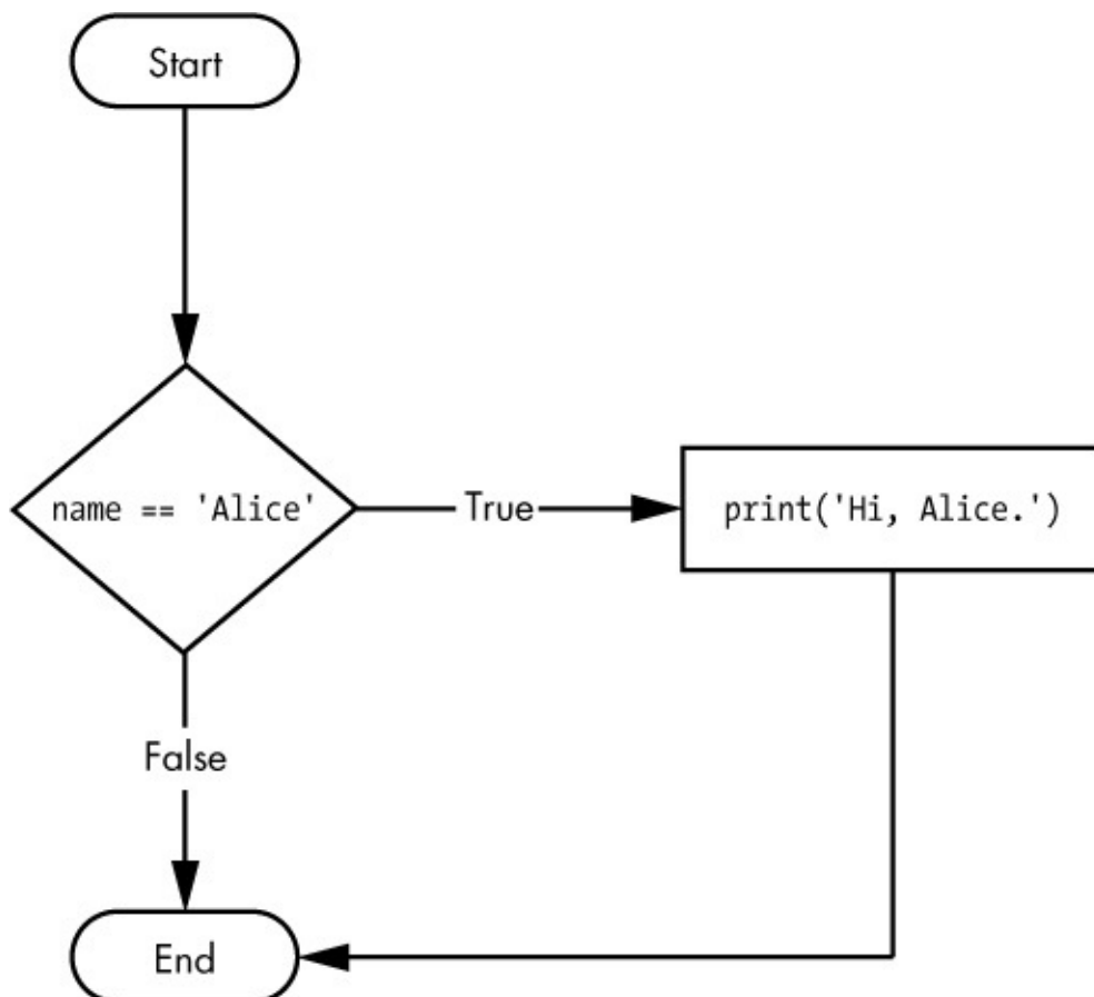
Figure 2-3. The flowchart for an if statement
