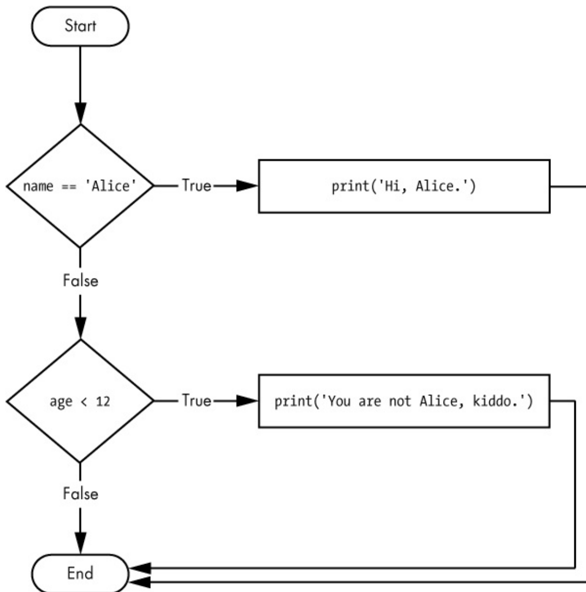
Figure 2-5. The flowchart for an elif statement
