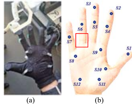
Fig. 1. Signals relative to grip force are sampled from 12 anatomically relevant FSR locations on the fingers and in the palm of both hands.
