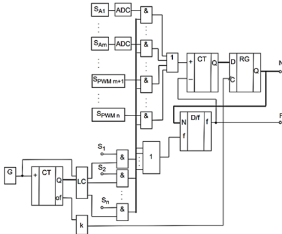
Fig. 1. Averaging pulse transducer.
