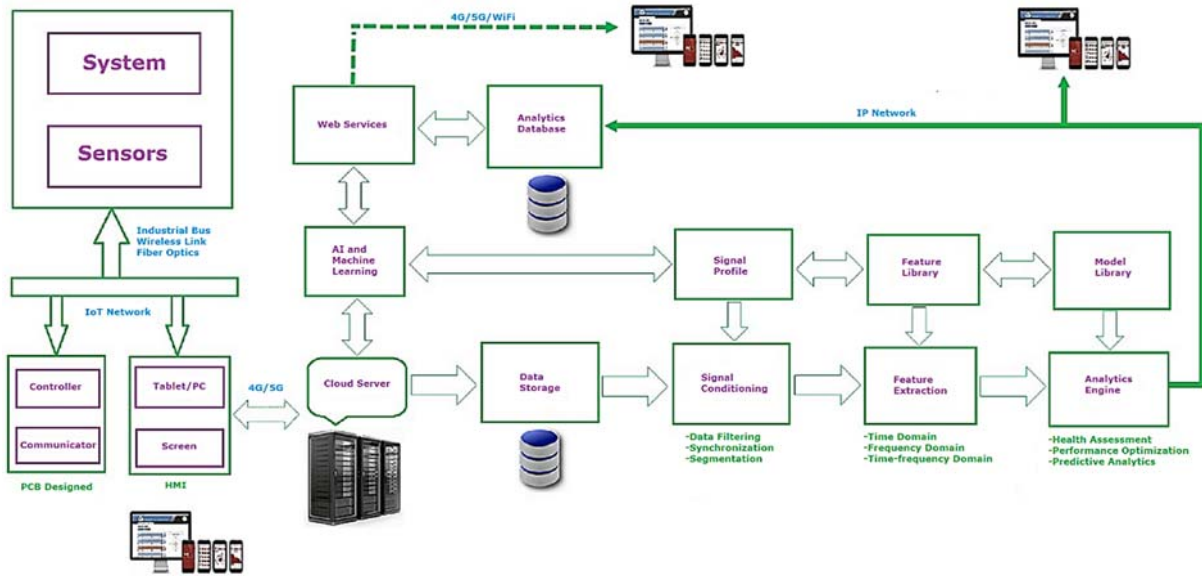
Fig. 1. Real-time machine learning system.
