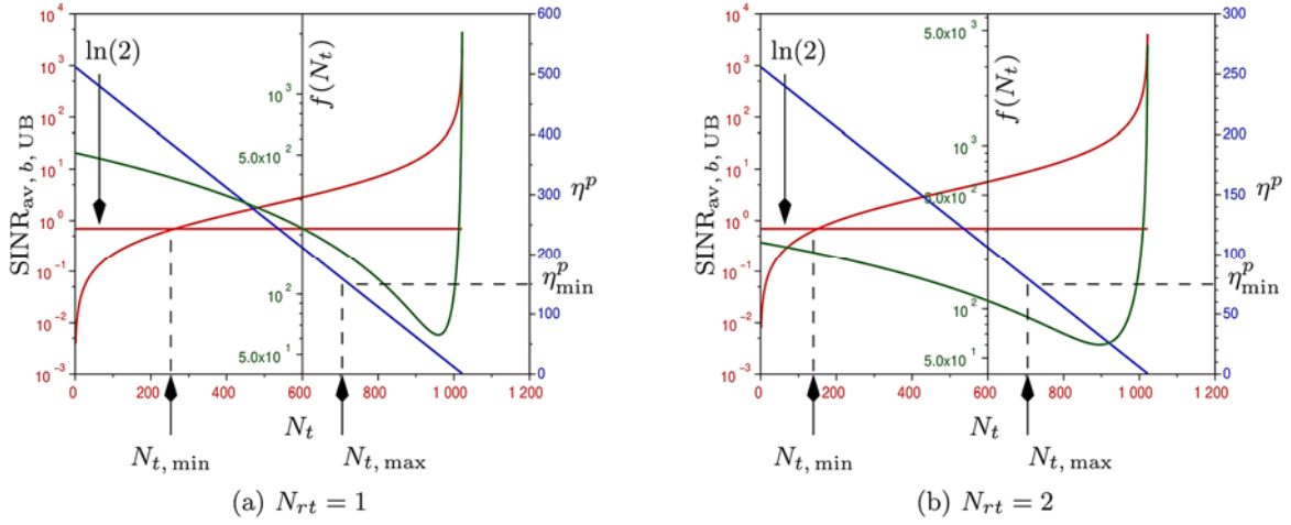
Fig. 2. SINR_{av, b, UB} and \eta^p as a function of N_t for N_{tot} = 1024 .
