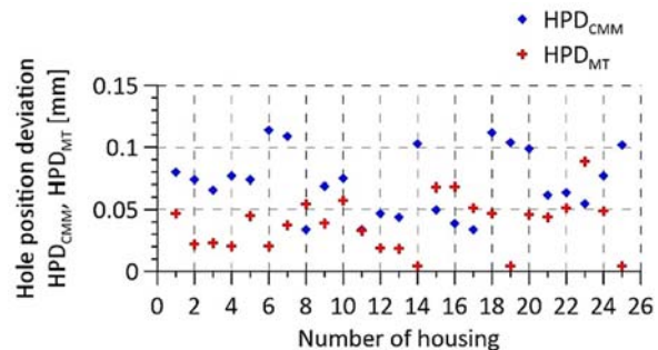
Fig. 3. Hole position deviations determined using the CMM and a machine tool.
