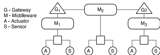
Fig. 2. Main middleware gateways concept.
