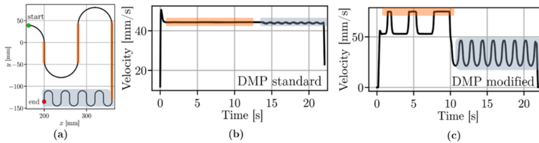
Fig. 6. Two different executions of the path shown in (a): in (b) the output velocity from a classical DMP formulation is presented, while in (c) the newly proposed method permits a continuous modulation of the velocity reference.
