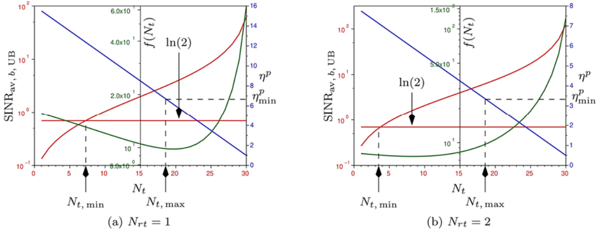
Fig. 3. SINR_{av, b, UB} and \eta^p as a function of N_t for N_{tot} = 32 .
