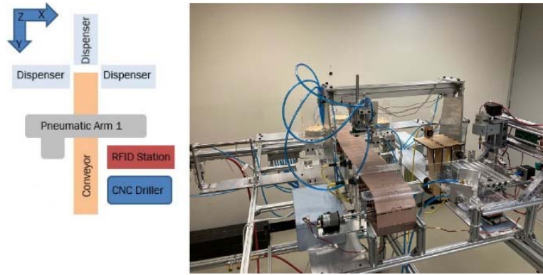
Fig. 1. Manufacturing cell.
