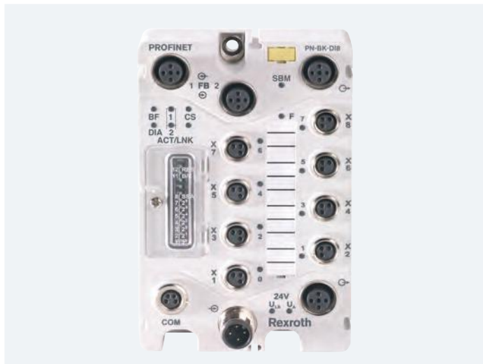
Fieldbus coupler – for connecting local I/O modules to a higher-level fieldbus system.
