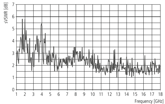
Typical performance Automotive 5 m (sVSWR)
