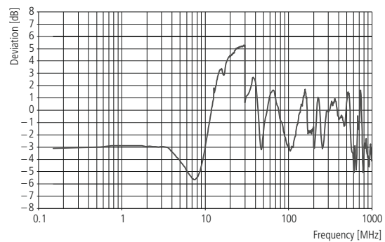
Deviation according to long wire measurement (LWM)
