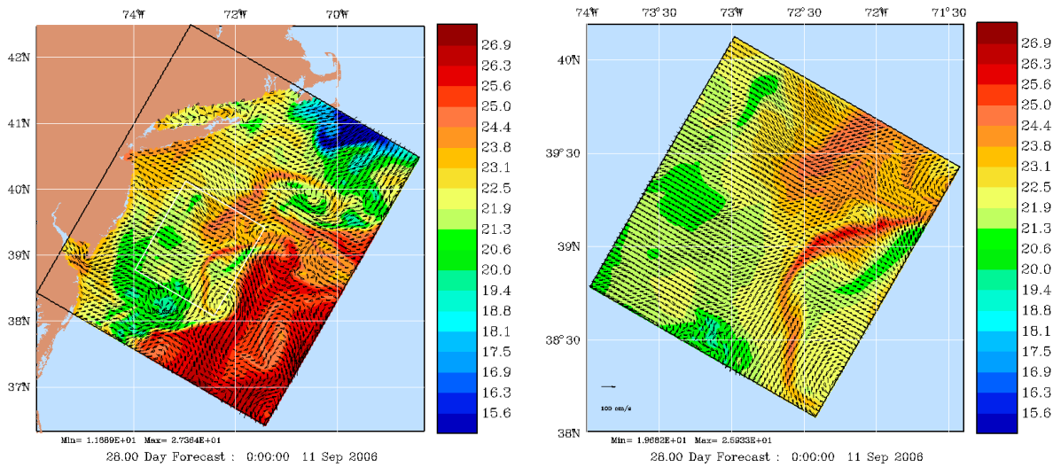
Figure 2. Surface temperature from the new nested reanalysis.
