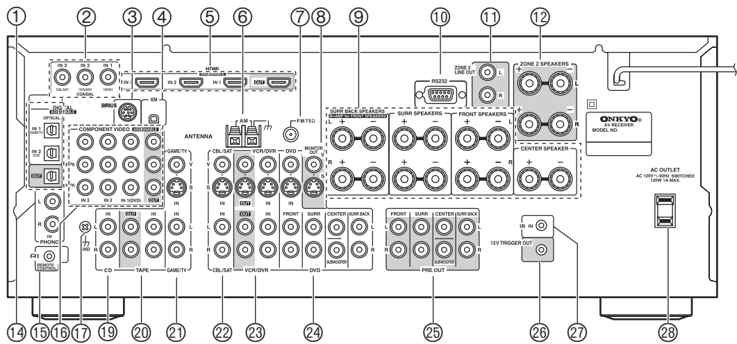
TX-SR705 other than North American model
