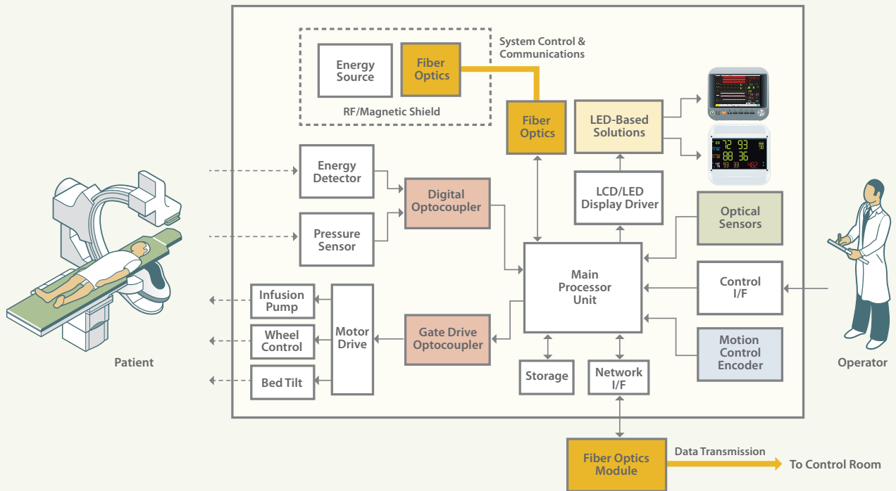
Typical Medical System Application Diagram
