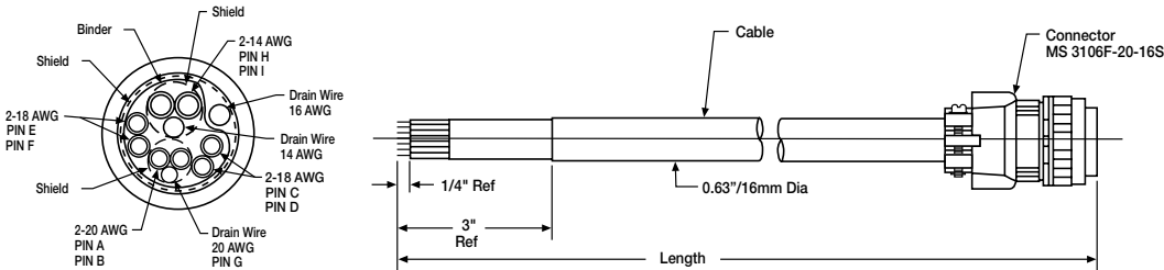
9 Pin
