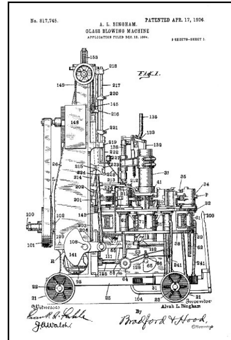
Figure 10 – Bingham’s 1906 patent
