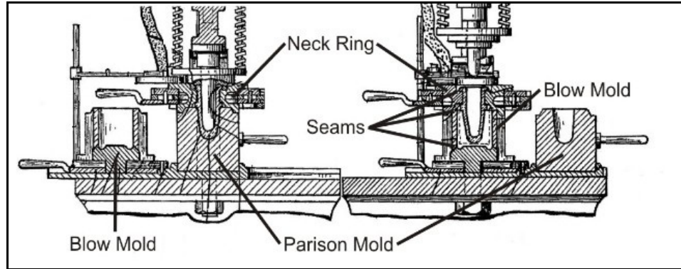
Figure 35 – Close view of molds from Haley-Bridgewater machine
