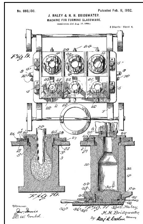
Figure 5 – Haley-Bridgewater 1902 patent
