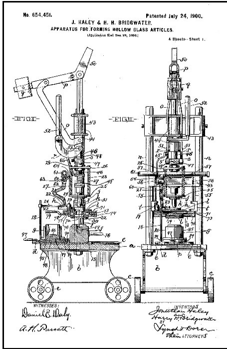
Figure 6 – Haley-Bridgewater 1900 patent
