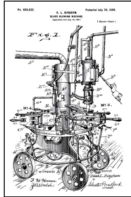
Figure 8 – Bingham’s 1898 patent
