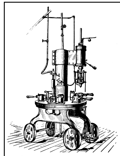
Figure 9 – F.C. Ball machine (Ball 1937:87)
