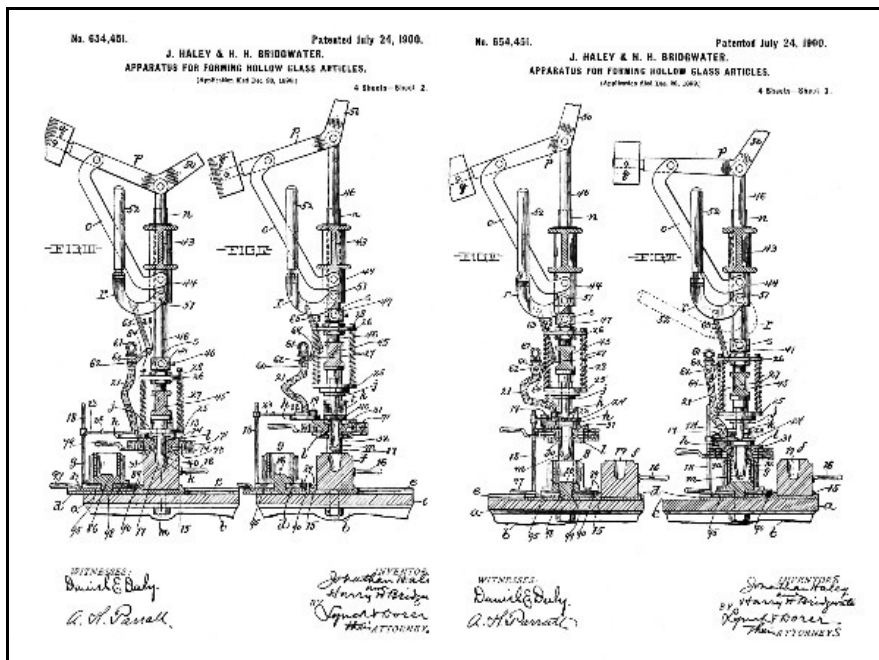
Figure 7 – Detail of Haley-Bridgewater 1900 patent
