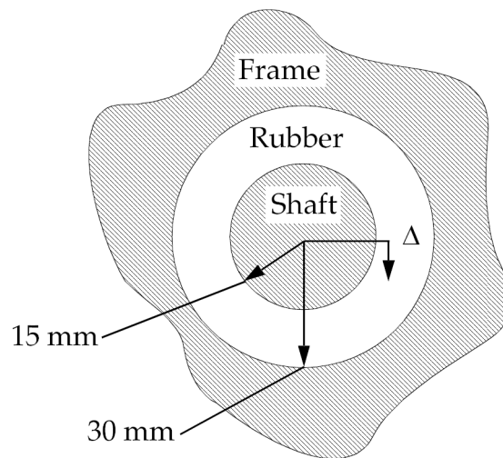
Figure 2-4. Rubber Bushing
