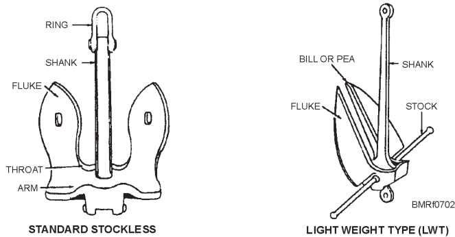
Figure 7-2.—Anchors.
