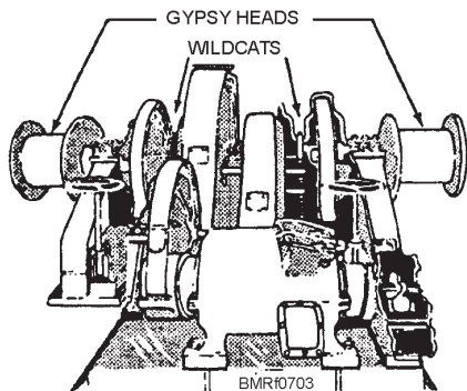
Figure 7-3.—Horizontal shaft anchor windlass.
