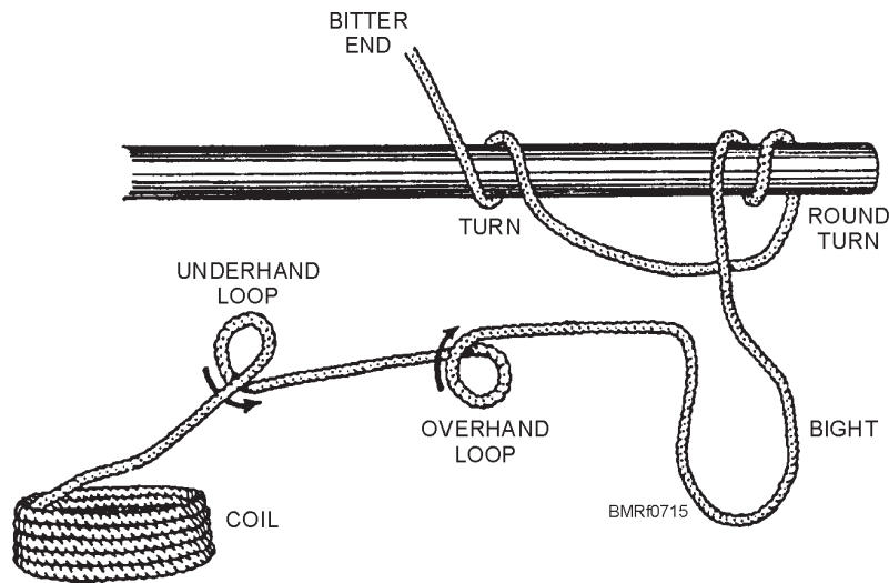
Figure 7-15.—Elements of knots, bends, and hitches.
