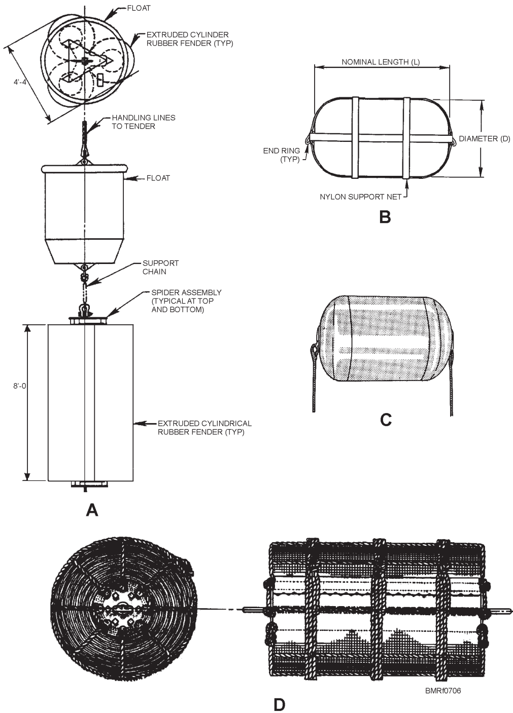
Figure 7-6.—Protection for the side of a ship.
