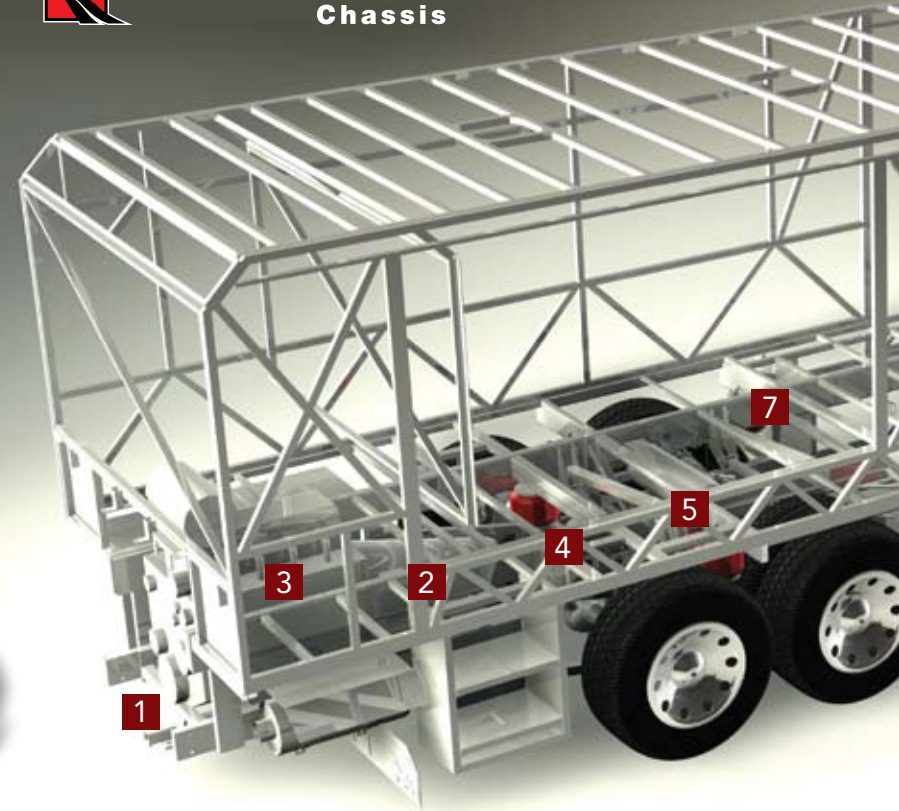
ROADMASTER S-SERIES SEMI-MONOCOQUE CHASSIS
