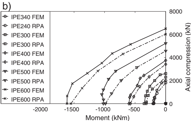
Fig. 11. Interaction diagrams resulting from the FEM analyses on the parametric beam sections.
