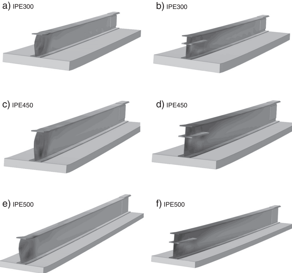
Fig. 16. Deformed configuration of three selected sections with and without longitudinal stiffeners (darker regions indicate larger stress concentrations but not necessarily yielding).
