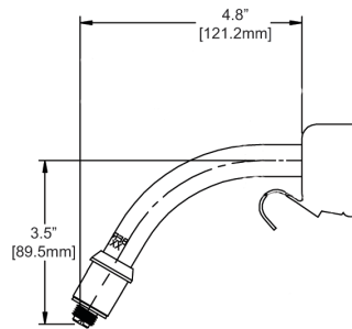
WC2T3-60 (60° Bend)
