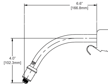
WC2T4-60 (60° Bend)
