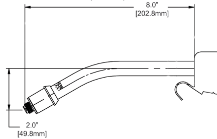
WC2T4-30 (30° Bend)
