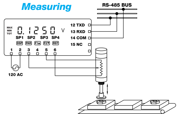
RS-485 BUS
