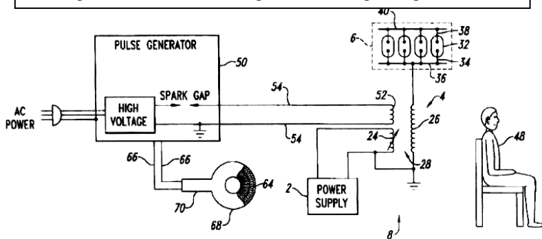
Figure 9 Diagram of Azure patent #6,217,604. “Method for treating diseased states ... using an electromagnetic generator”
