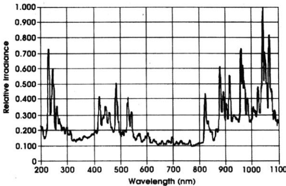
Figure 11 Spectrum of xenon gas
