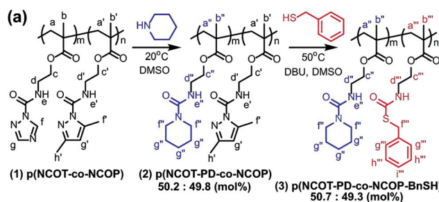
Fig. 6 Polymers with pendent blocked isocyanate groups sequentially modified through the exploitation of different deblocking temperatures between the pyrazole and the triazole. Reprinted from ref. 93. Copyright 2016 American Chemical Society.
