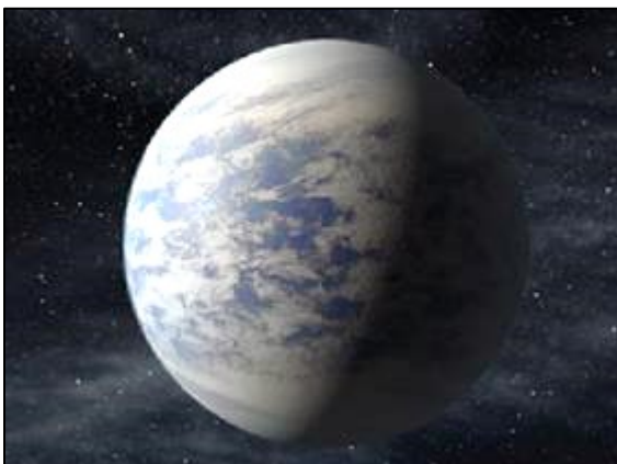
Artist’s Rendition of “Earth-Like” Planet Kepler-69c.
