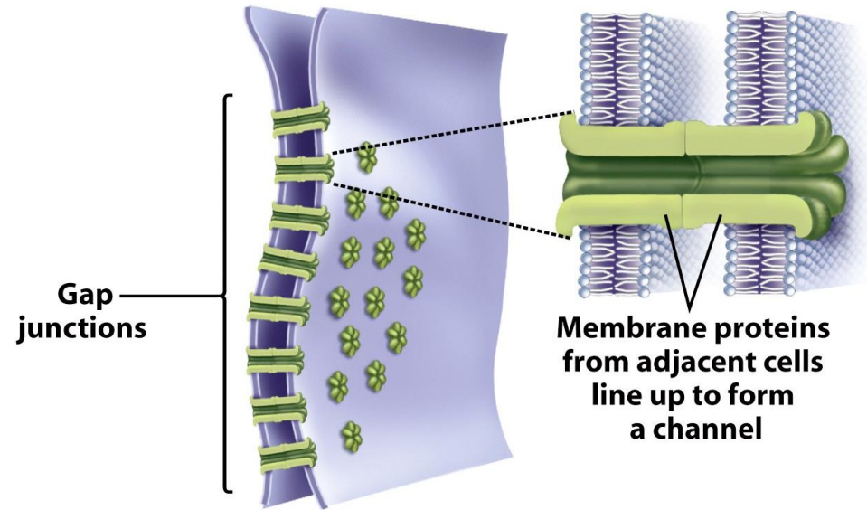
Fig.19: Gap junction
