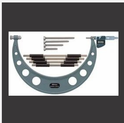
Mitutoyo Outside Micrometers Series 340
