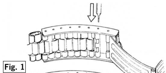
Multiple Band Sizing Tool (S-926)
