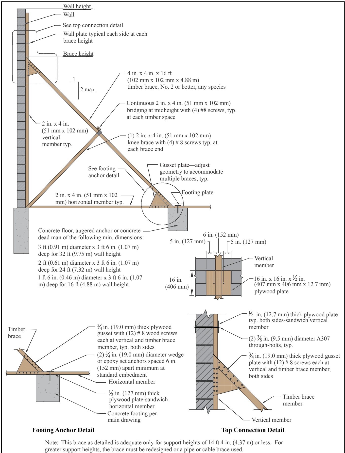
Figure 2—Wood Brace Detail
