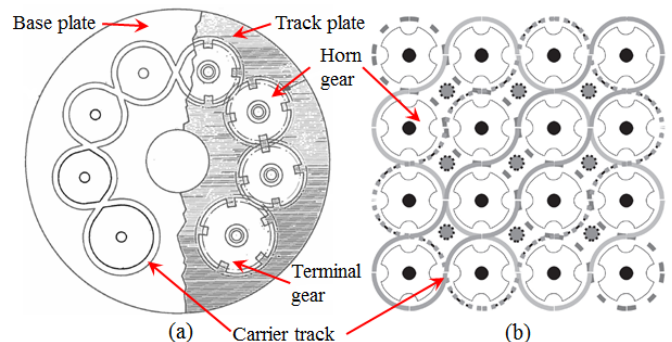
Fig. 4: Schematic of (a) flat braider carrier track[8] (b) profile (2.5D) braider with four tracks[9] also known as 4x4 braider
