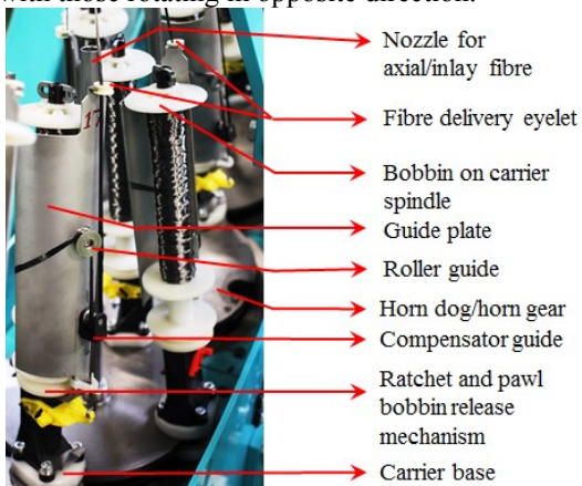
Fig. 3: Different components of a radial braider carrier
