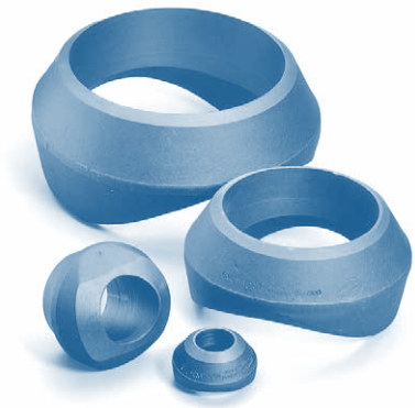
Design per MSS SP-97 BW ends per B16.9 and B16.25 Each outlet size listed is available to fit any run curvature.
