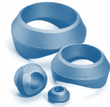
Design per MSS SP-97 BW ends per B16.9 and B16.25 Each outlet size listed is available to fit any run curvature.
