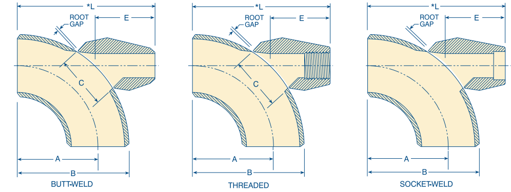
FOR ELBOW OUTLETS THREADED, SOCKET-WELD AND BUTT-WELD ENDS
