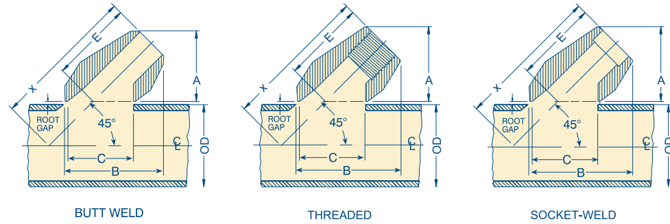
45° BRANCH CONNECTIONS THREADED, SOCKET-WELD AND BUTT-WELD ENDS
