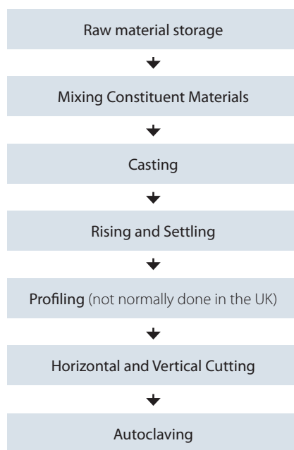
Figure 7: The aircrete process
