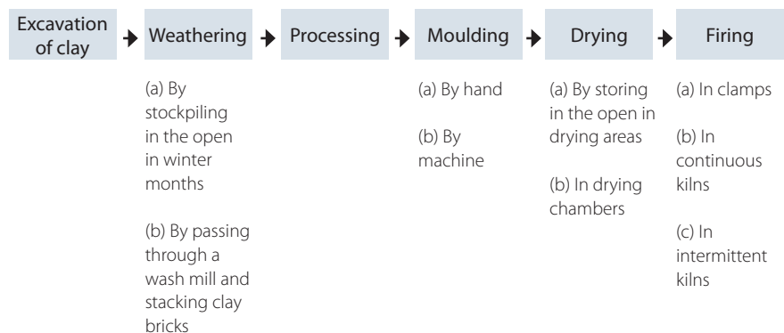
Figure 3: Clay brick production
