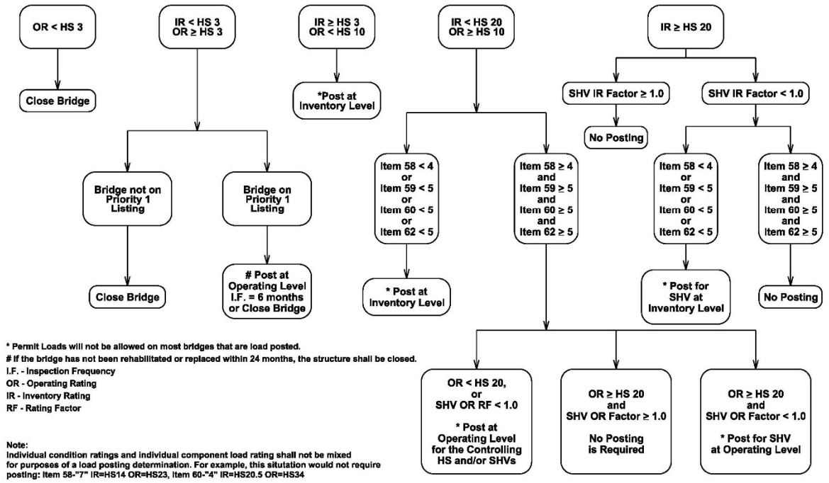
Figure 6-4. On-System Load Posting Guidelines
