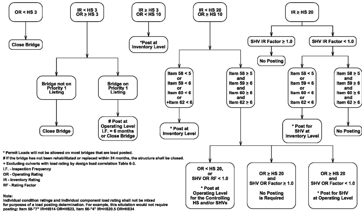
Figure 6-5. Off-System Load Posting Guidelines
