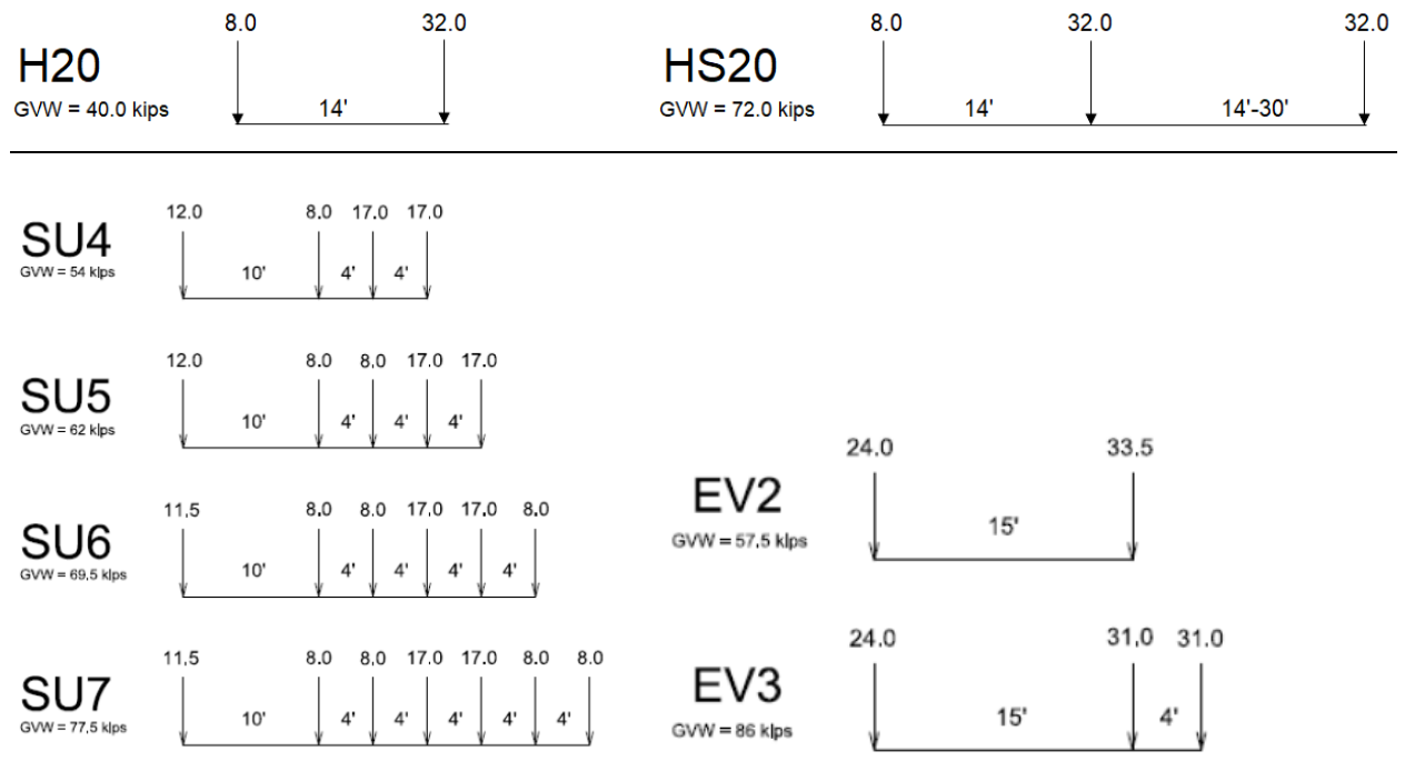
Figure 6-3. H, HS, SHV and EV Truck Load Configurations
