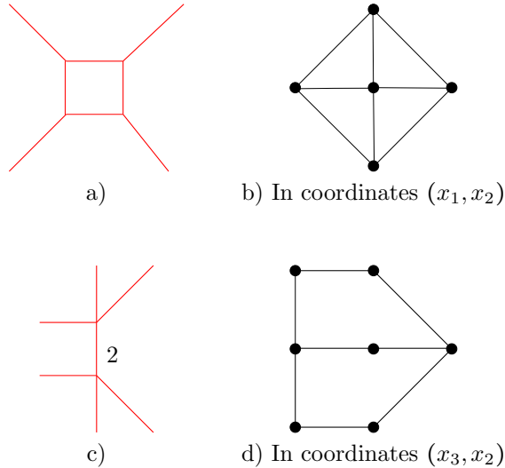
FIGURE 32. The two tropical limits of the curve in Example 5.32 with respect to the two coordinate systems. Beside them are the respective subdivisions of their Newton polygons.
