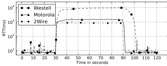
(a) Empirical measurements of modem buffering. Different modems have different buffer sizes, leading to wide disparities in observed latencies when the upstream link is busy. (BISMark)
