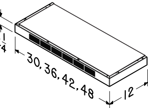
A non-duct kit may be used to recirculate filtered air back into the kitchen if ducting is not practical.
