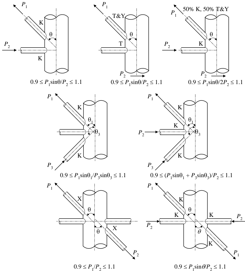
FIGURE 2 Examples of Tubular Joint Categorization
