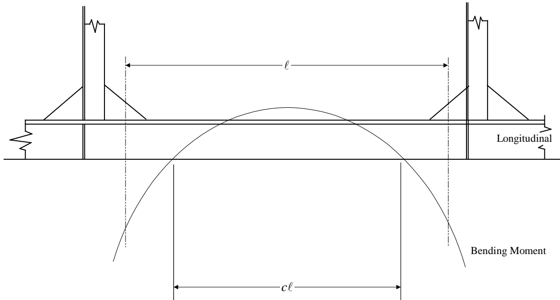
FIGURE 8 Effective Breadth of Plating s_w
