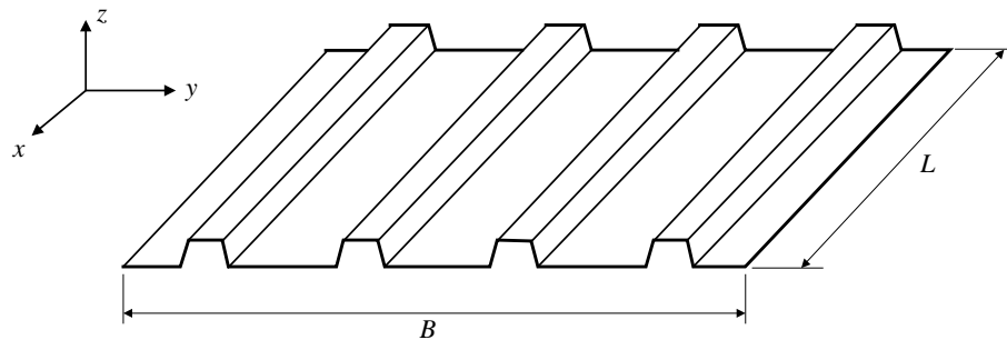
FIGURE 3 Typical Corrugated Panel
