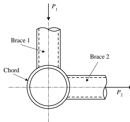
FIGURE 4 Multiplanar Joints
