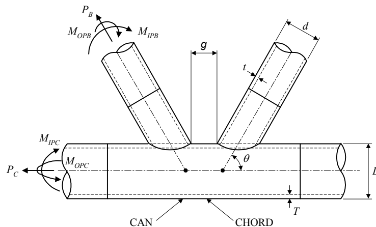
FIGURE 1 Geometry of Tubular Joints
