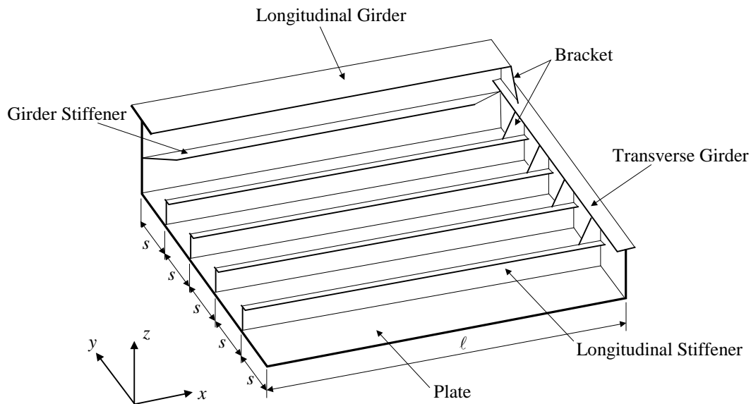
FIGURE 1 Typical Stiffened Panel
