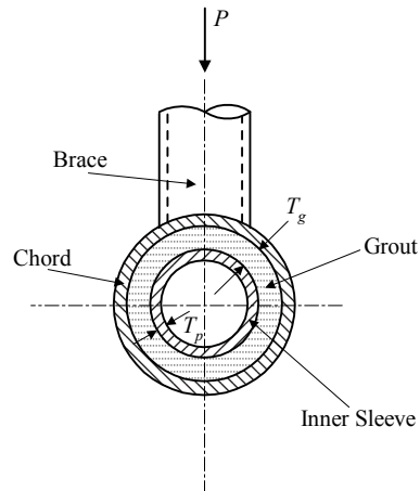
FIGURE 5 Grouted Joints
