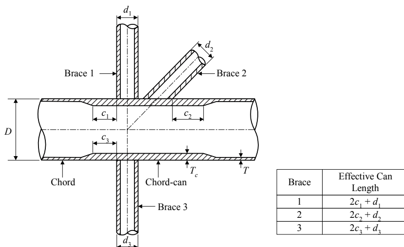
FIGURE 3 Examples of Effective Can Length
