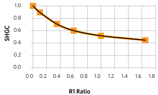
Curve Fit for South Horizontal Shades
