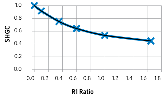
Curve Fit for West Horizontal Shades
