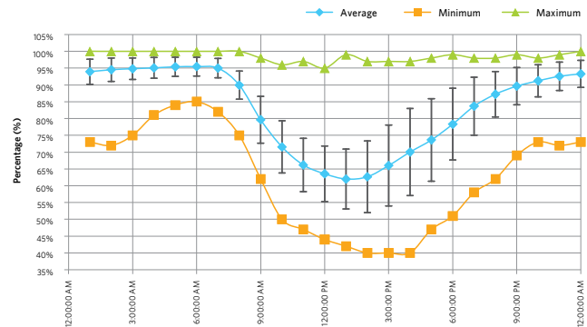
CHART 2.6 | RELATIVE HUMIDITY
