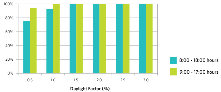
CHART 4.3 | PERCENTAGE OF HOURS WHERE THE DAYLIGHT FACTOR OF DIFFUSE LIGHT EXCEEDS 300 LUX LEVEL
