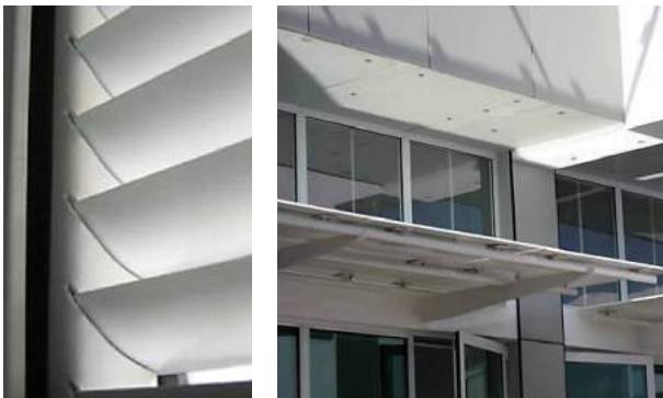
FIGURE 4.4 | EMBEDDED BLINDS IN DOUBLE GLAZING WITH EXTERNAL LIGHT SHELVES (GEO BUILDING, MALAYSIA)
