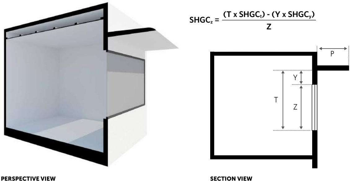
FIGURE 6.3.2.4 | SOLUTION TO CALCULATE THE SHGC OF FENESTRATION WITH OFFSET HORIZONTAL PROJECTIONS
