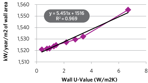
Peak Cooling Load
