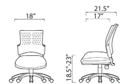
Low back chair without armrest
