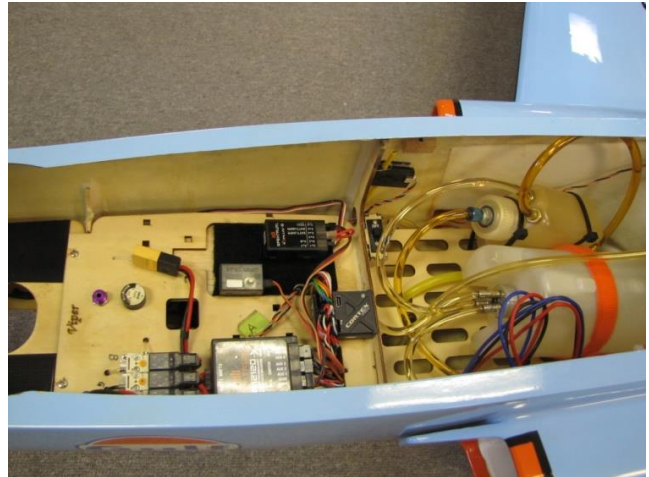
View of right side of mid forward fuse. See optional channel expander, flight logger, mini air pressure gauge, air fill valve, and Cortex Gyro.
