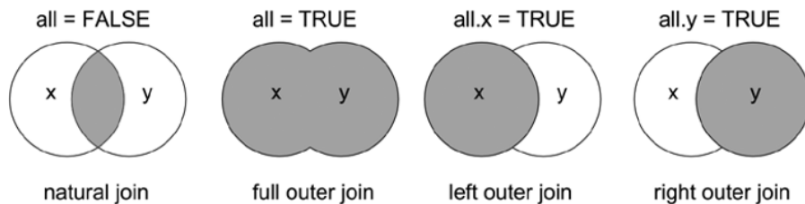
Figure 13-2: Different types of merge() and their database join equivalents.
