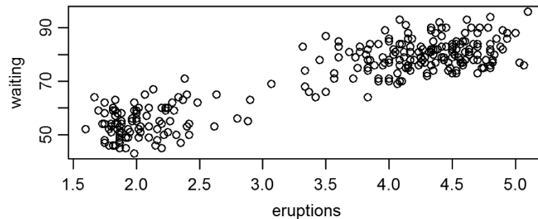
Figure 16-2: Creating a scatterplot.
