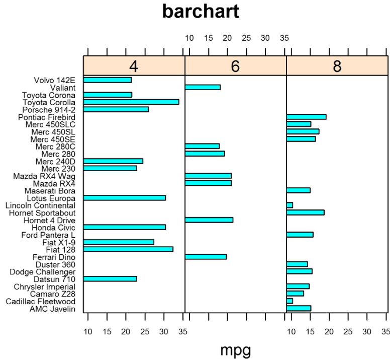
Figure 17-7: Making a lattice bar chart.
