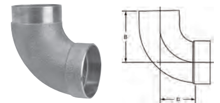
807-2 \triangle DWV 90° Fitting Elbow Ftg x C – Cast
