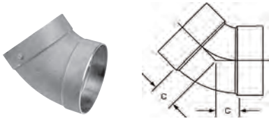
806 \triangle DWV 45° Elbow C x C – Cast
