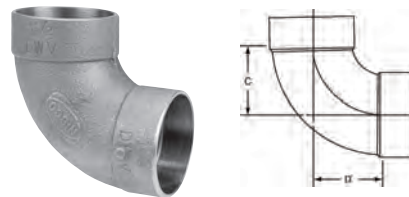
807 \triangle DWV 90° Elbow C x C – Cast
