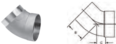
806-2 \triangle DWV 45° Fitting Elbow Ftg x C – Cast
