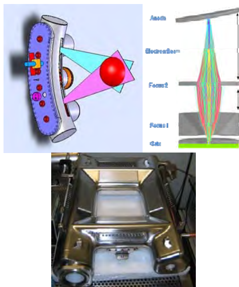
Figure 14 Schematics showing a nanotube x-ray source array (top) and a square-geometry nanotube x-ray source array with 52 individually controllable x-ray beams (Figure courtesy of XinRay Systems).
