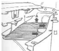
Fig. 319 Cabin air filter removal. 1998-2005 Volkswagen New Beetle
