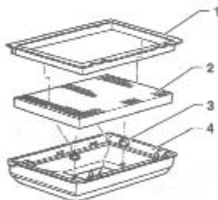
Fig. 319 Cabin air filter removal. 1998-2005 Volkswagen New Beetle
