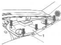
Fig. 318 Righthand close-out panel attaching screw locations. 1998-2004 Volkswagen New Beetle
