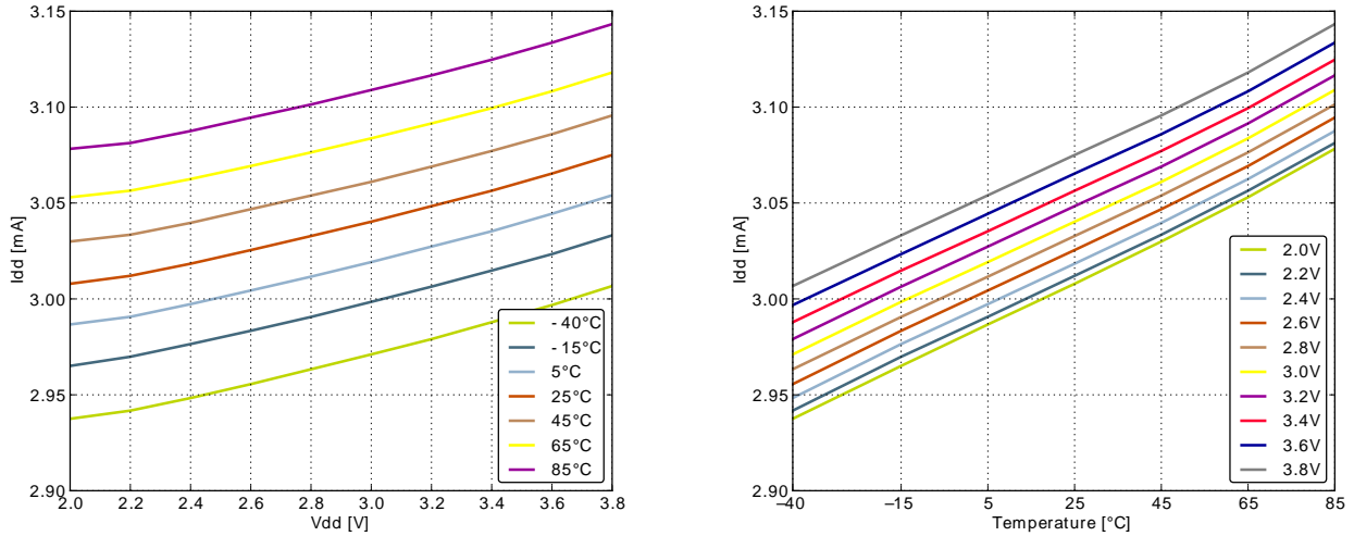
Figure 3.2. EM1 Current consumption with all peripheral clocks disabled and HFRCO running at 28MHz
